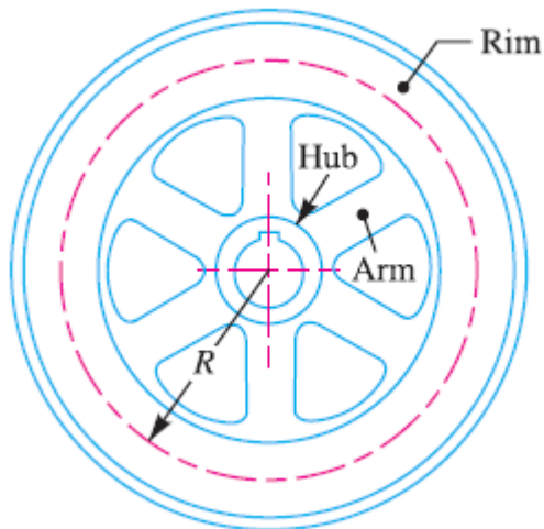
Fig. 4 Flywheel
