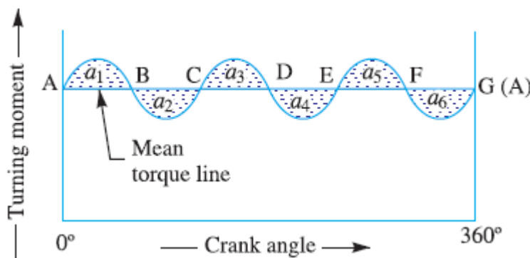
Fig. 3 Turning moment diagram for a multi-cylinder engine
