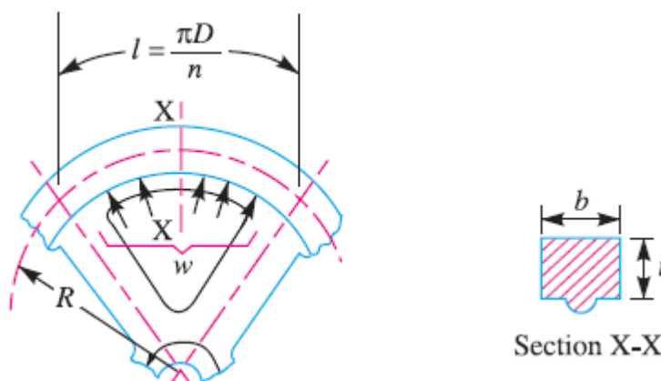
Fig.6 One section of the flywheel rim
