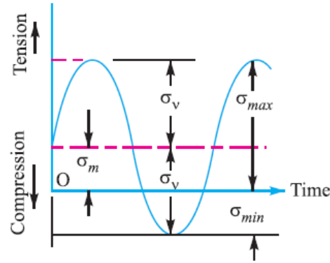
Fig. 5 fluctuating stress
