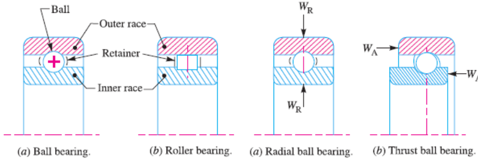
Fig. 3 Ball and Roller Bearing
