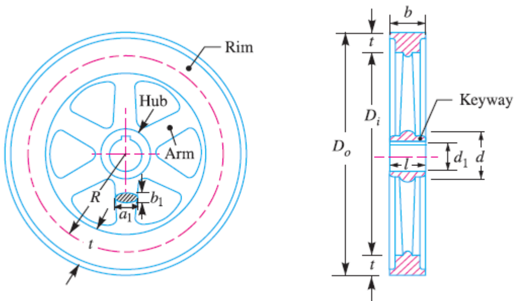
Fig. 5 Different dimensions of flywheel
