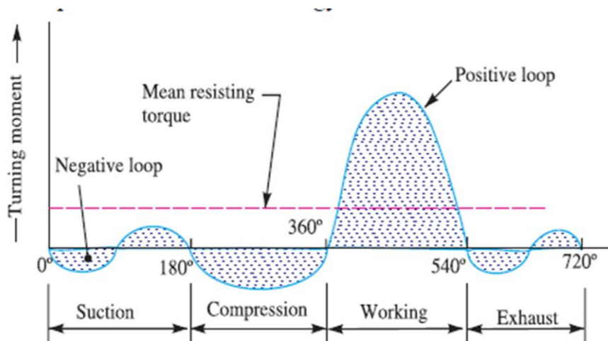
Fig. 2 Turning moment diagram for a four stroke internal combustion engine
