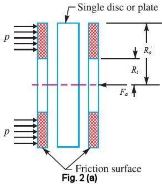
Fig. 2 Forces on the disc
