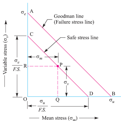
Figure 10 Goodman method
