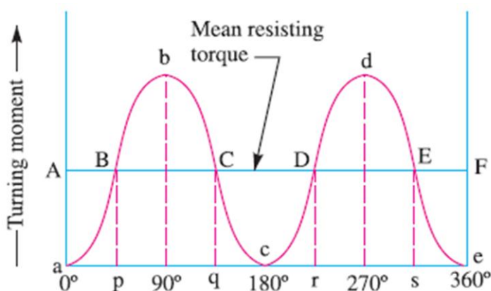
Fig. 1 Turning moment diagram of single cylinder double acting steam engine
