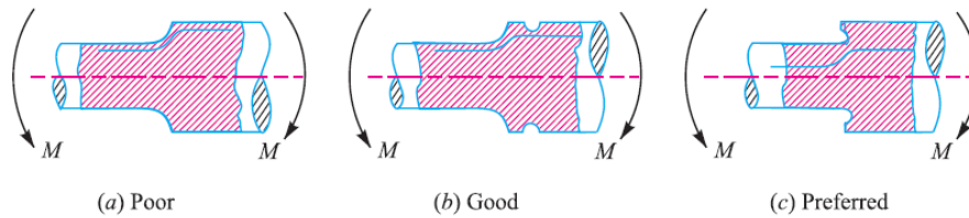
Figure 8 Notches to improve stress concentration Fatigue Stress Concentration Factor
