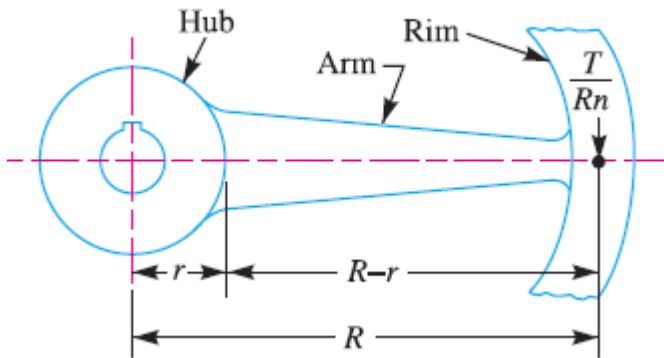
Fig.7 Arm cross-section of the rim
