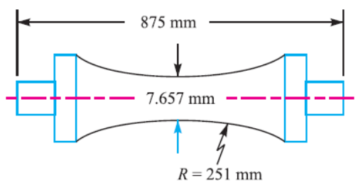
Fig. 2 standard specimen
